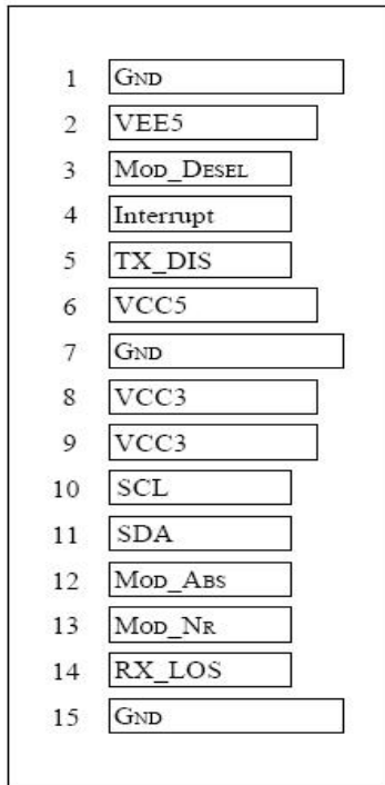
Bottom of Board (As view through top of board)
